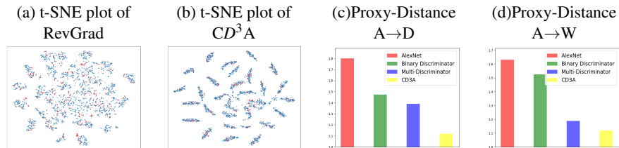
Figure 3: (a) and (b) figures show t-SNE visualizations of the CNN’s activation (a) in case when adapted through[10] and (b) when adapted through proposed model. Blue and red points correspond to the source domain(A), and the target domain (W) respectively. Sub figures (c) and (d) show the proxy distance for A→D and A→W.
